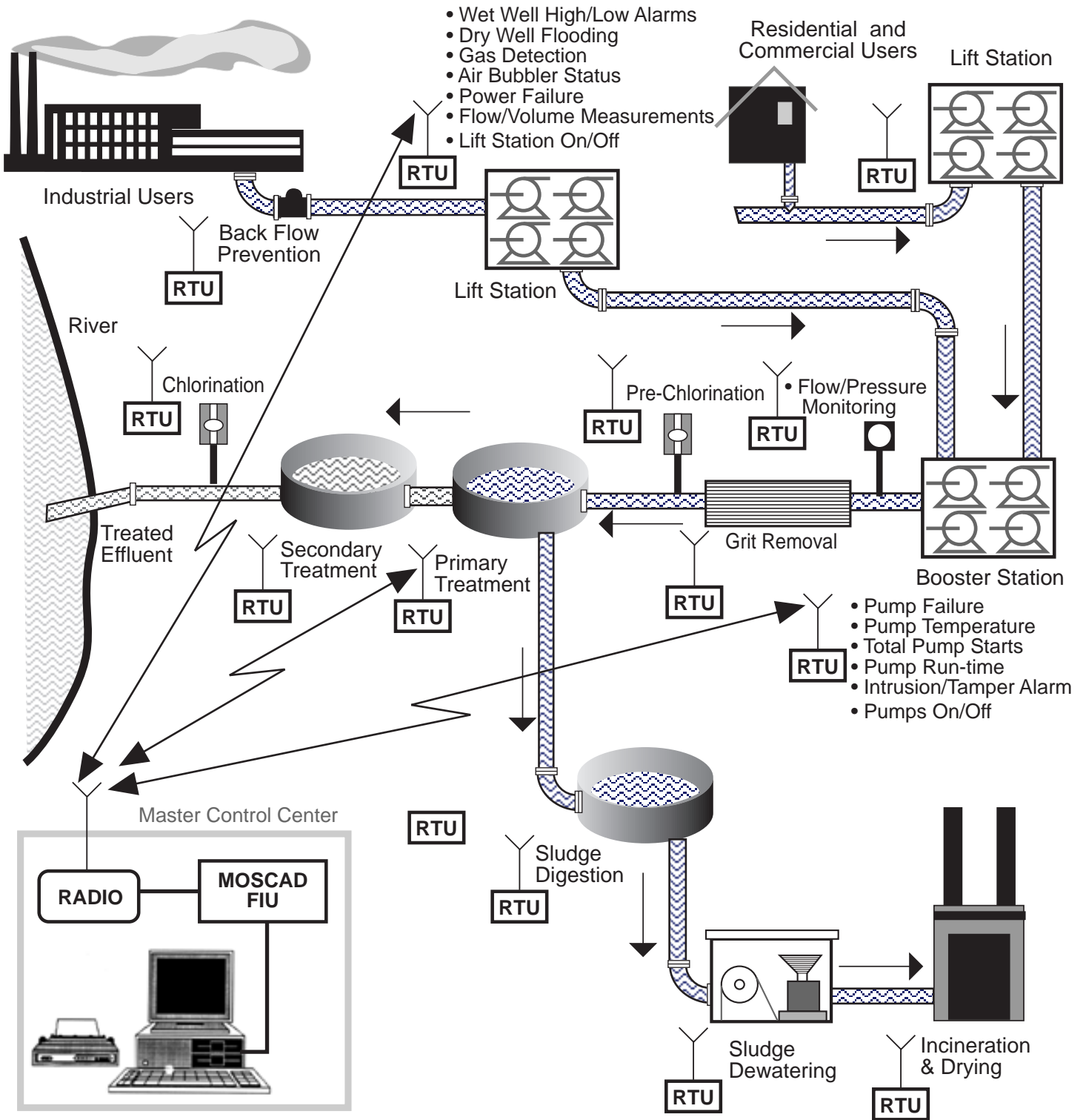
Fig. 2. TYPICAL WASTEWATER CONTROL SYSTEM
